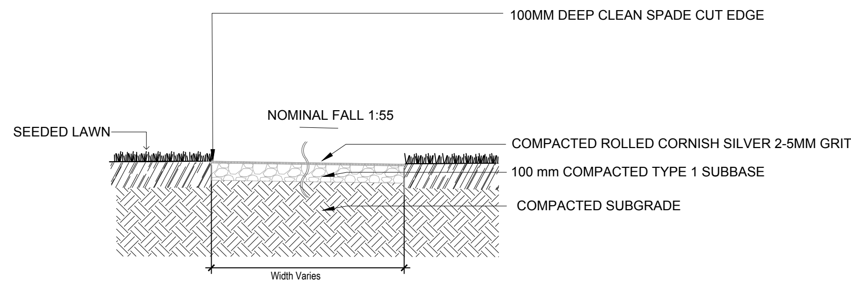
04 3001 SINGLE LAYER GRAVEL PATH WITH CUT EDGE DETAIL 1:20
