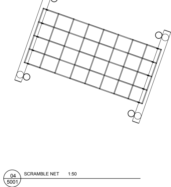
04 5001 SCRAMBLE NET 1:50
