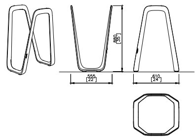
09 BICYCLE STAND 1:50 5002
