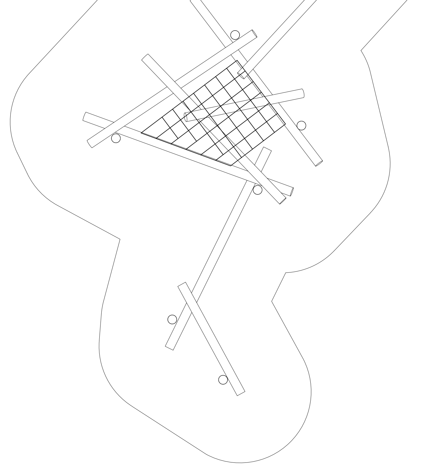
06 5001 CLAMBER STACK 1:50
