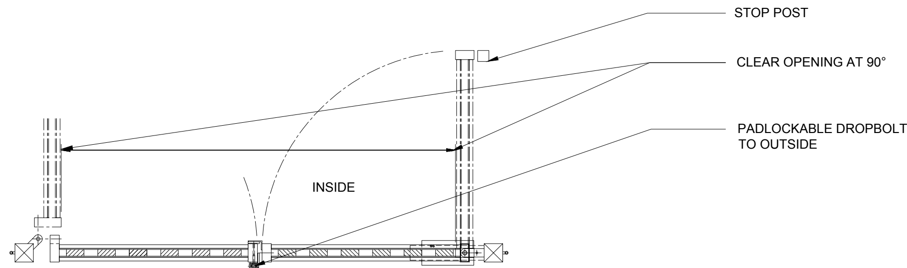
PLAN
