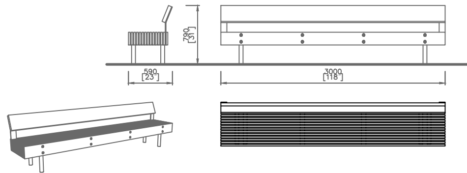
01 BACKED BENCH 1:50 5002
