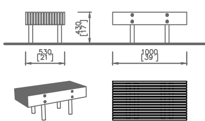
03 BACKLESS BENCH 1M 1:50 5002
