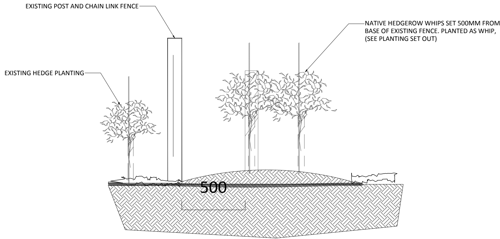
SECTION VIEW
