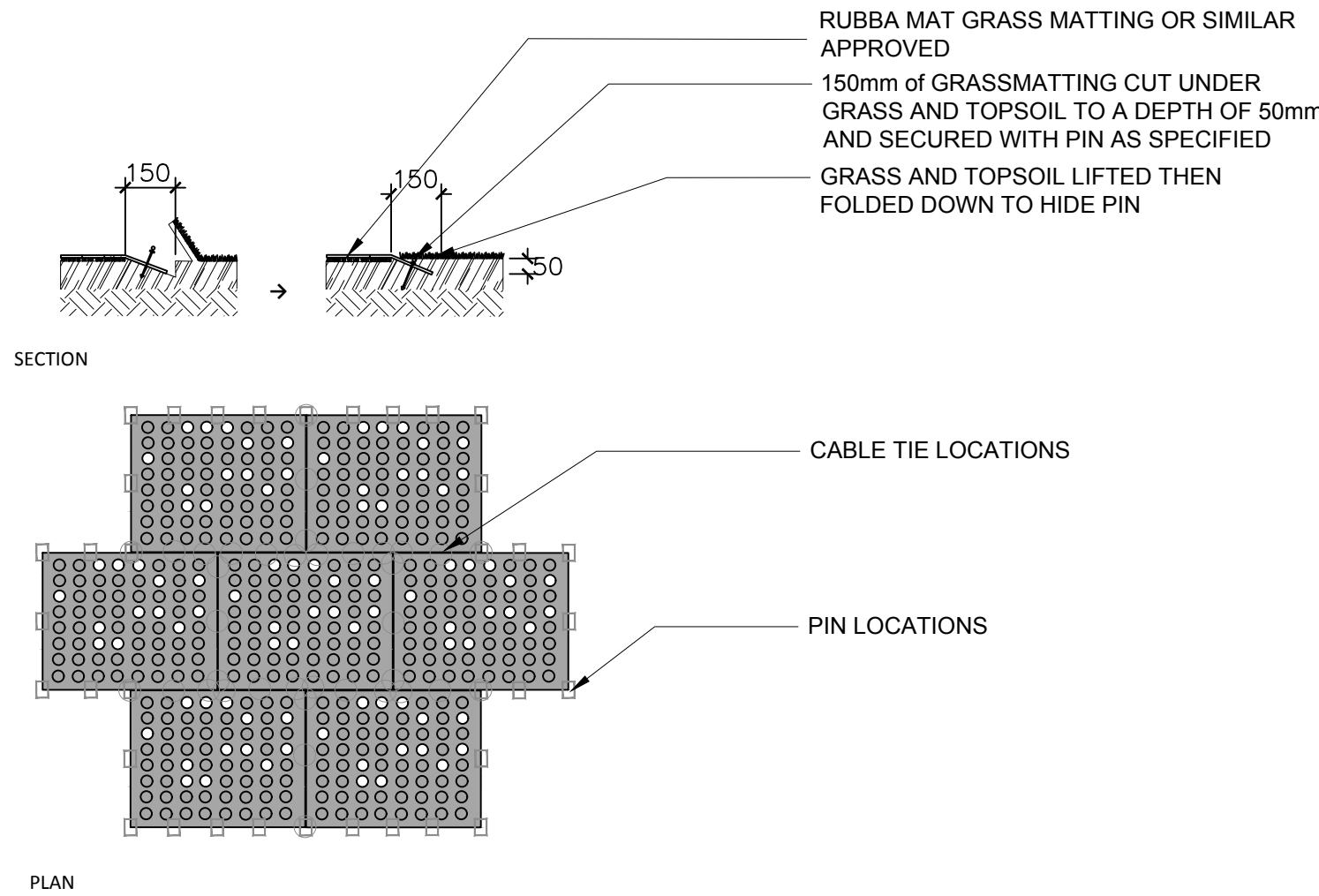
05 3001 RUBBER GRASS MAT SAFETY SURFACE DETAIL 1:20
