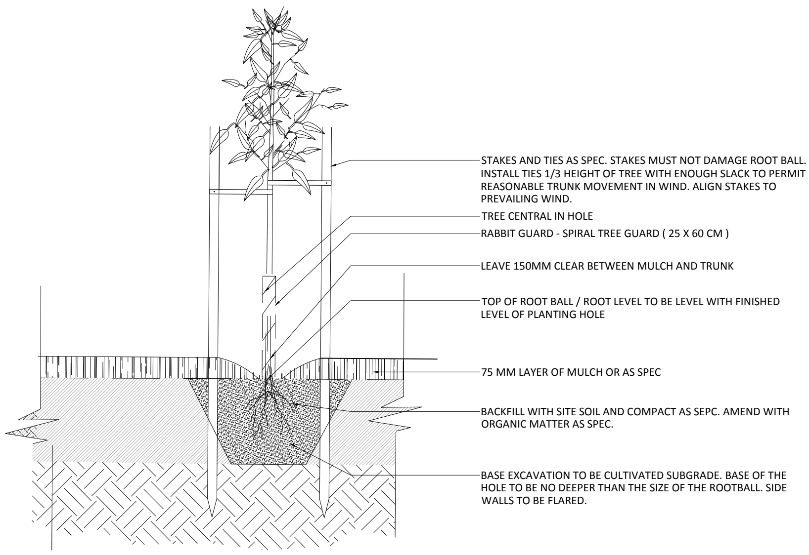
03 4001 FEATHERED BAREROOT TREE PLANTING DETAIL 1:20
