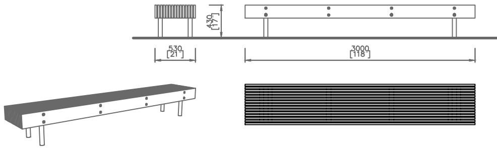
02 BACKLESS BENCH 1:50 5002
