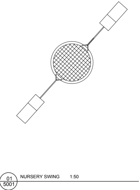
01 5001 NURSERY SWING 1:50
