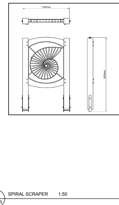
11 5001 SPIRAL SCRAPER 1:50
