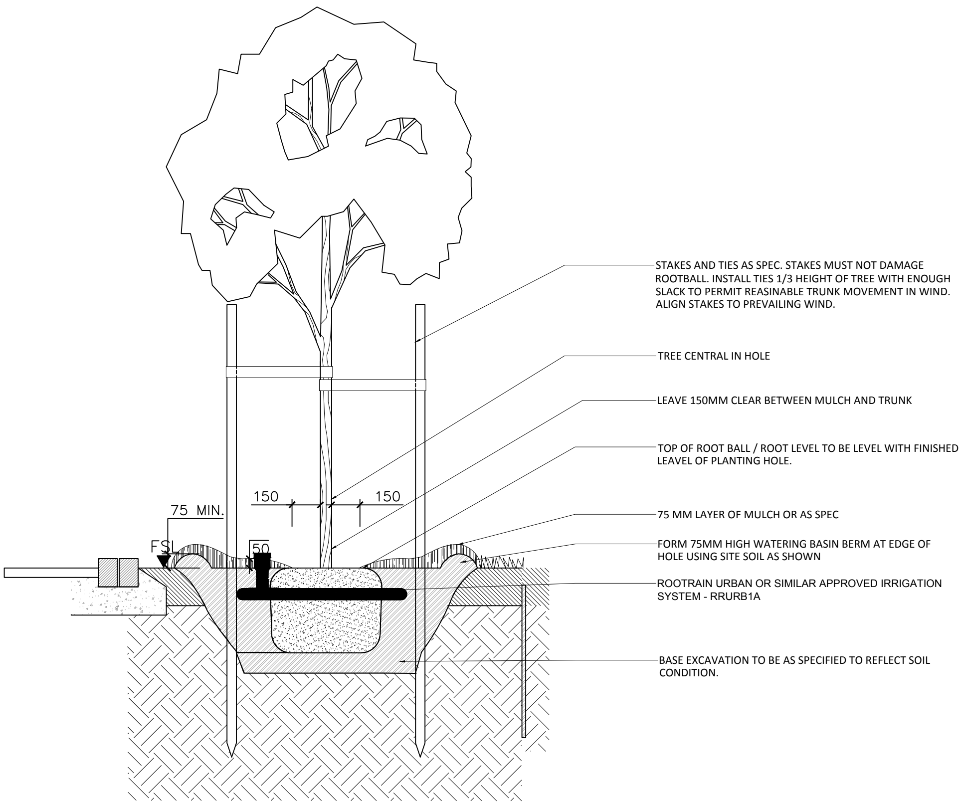
02 4001 STANDARDLIGHT STANDARD TREE PLANTING IN SOFT LANDSCAPING DETAIL 1:20
