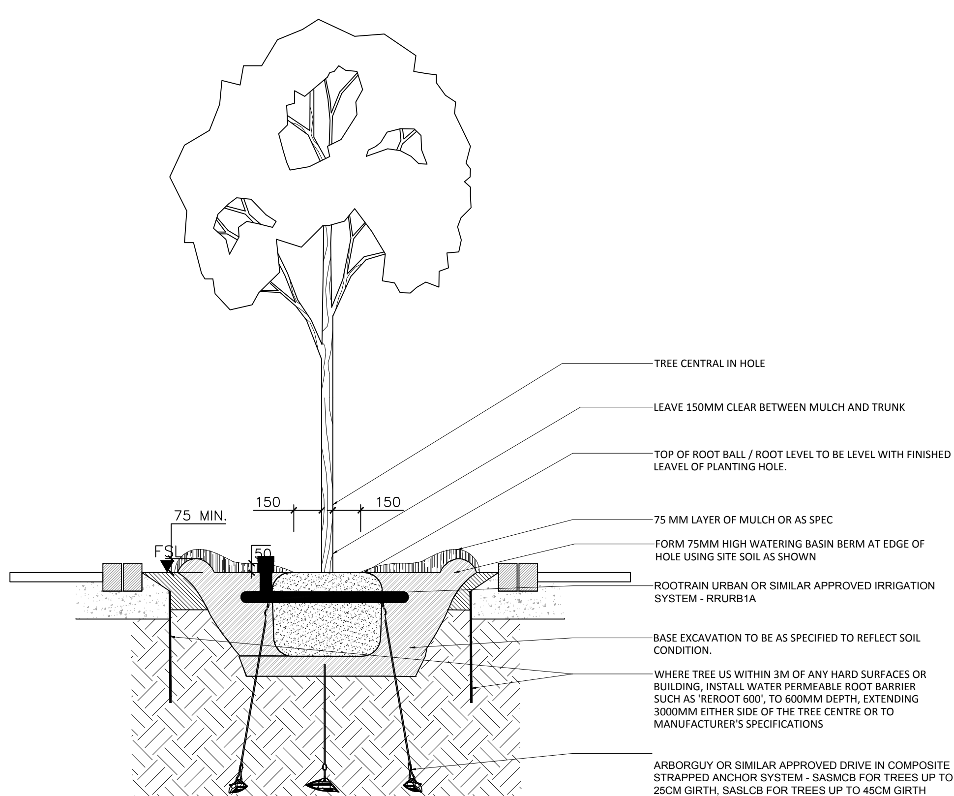
01 4001 STANDARDLIGHT STANDARD TREE IN HARD LANDSCAPING PLANTING DETAIL 1:20
