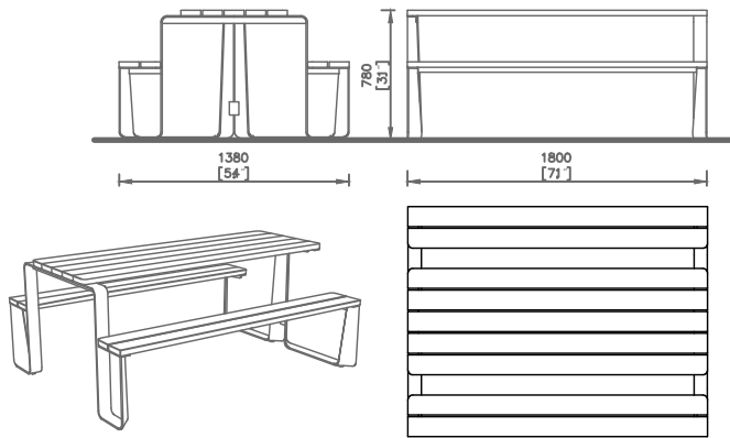
04 PICNIC BENCH AND TABLE SET 1:50 5002
