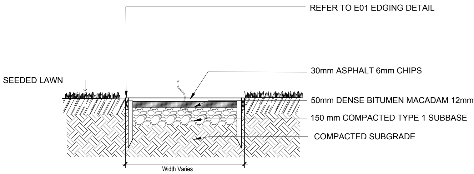
01 3001 ASPHALT PATHWAY WITH TIMBER EDGING DETAIL 1:20
